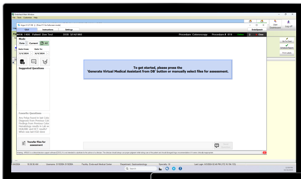
Windows-Based
